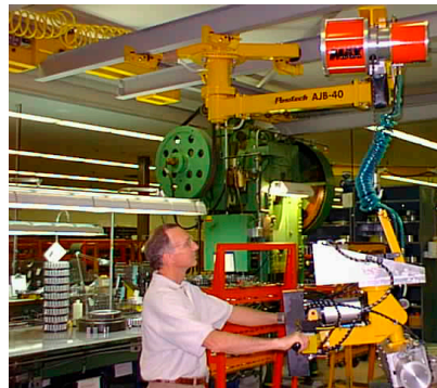
Trolley mounted AJB with balancer handling a bearing race.
