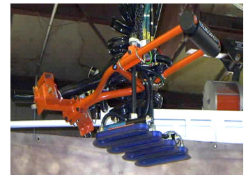
Hook hung vacuum end-effector with extended pivoting handle.
